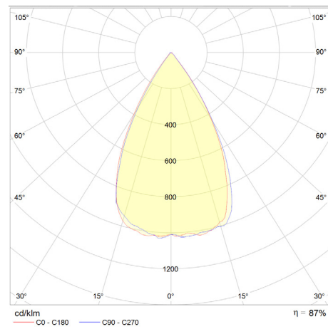
LUXEON 3030 2D
